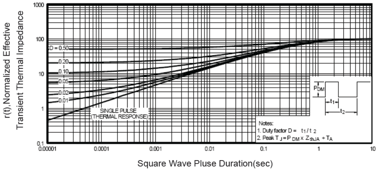
图 14 Normalized Maximum Transient Thermal Impedance
